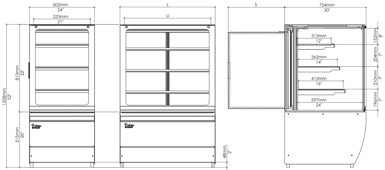
600 Front Elevation
