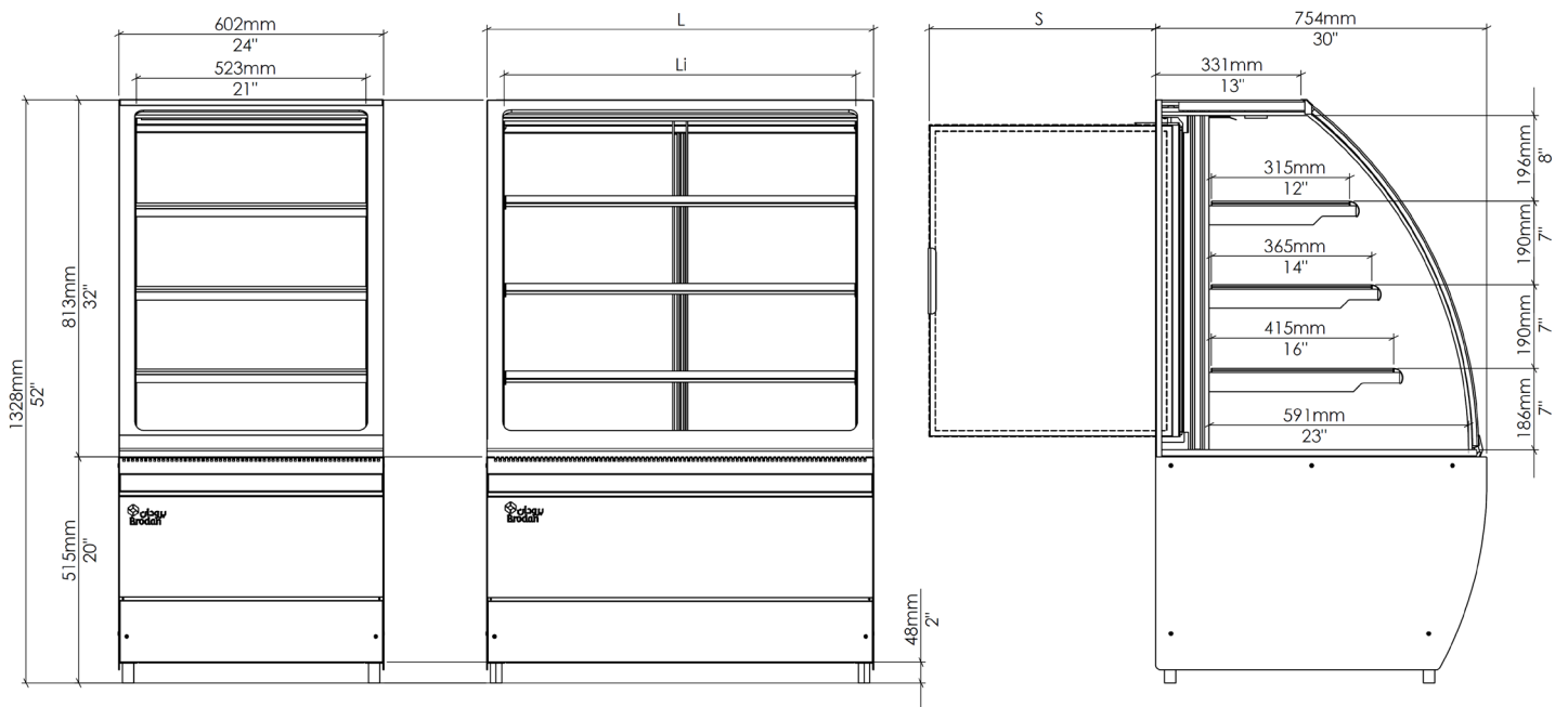
600 Front Elevation
